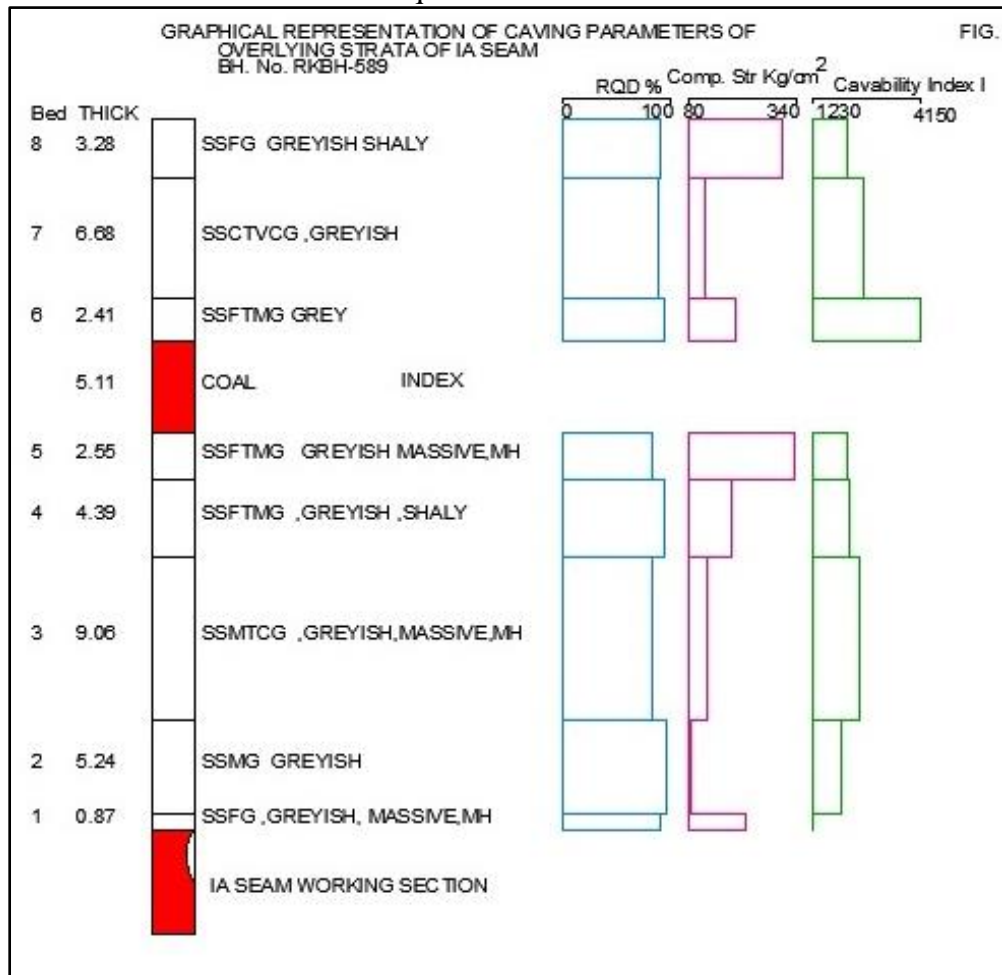
Figure 4 Graphical representations of Caving Parameters of Overlying Strata of BH. No. RKBH-589
